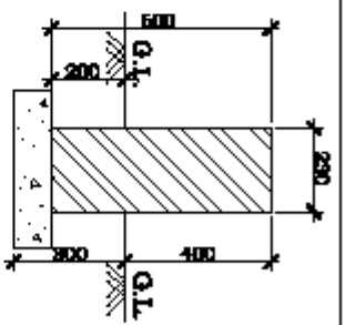
CROSS SECTION OF A - A
